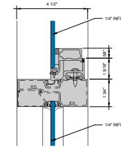
② GLASSVENT SILL @ HORIZONTAL 6" = 1'-0"
