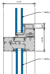
① GLASSVENT SILL @ HORIZONTAL Ø = 1" Ø
