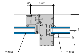
② GLASSVENT JAMB @ VERTICAL Ø = 1" Ø
