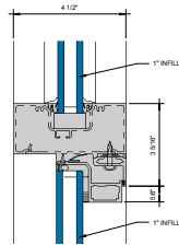
① GLASSVENT HEAD @ HORIZONTAL Ø = 1" Ø
