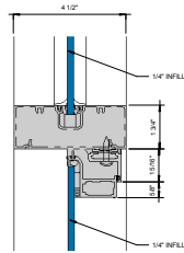
① GLASSVENT HEAD @ HORIZONTAL 6" = 1'-0"
