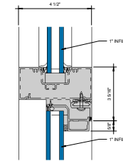
② GLASSVENT HEAD @ HORIZONTAL Ø = 1" Ø
